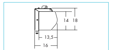
Trigger cable
