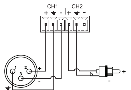
Balanced - XLR
